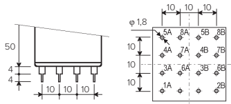
Hole layout (from solder side)
