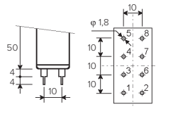
Hole layout (from solder side)
